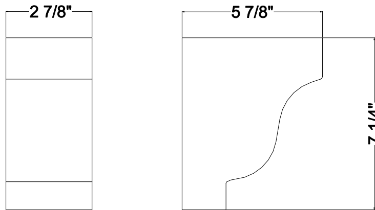
ITEM NUMBER:COR05X02X07TR 2 7/8"W x 5 7/8"D x 7 1/4"H Traditional Corbel
